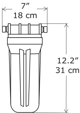
pH Neutralizer D = 4.7" / 12 cm
