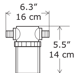
Sea Strainer D = 3.8" / 9,5cm
