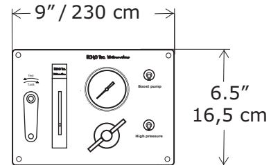
Control Panel D = 5" / 12,7 cm
