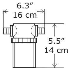
Sea Strainer D = 3.8" / 9,5cm
